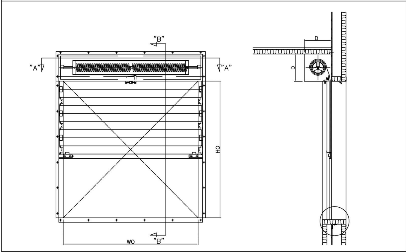
Fire Shutter
