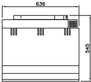
Plan View – 2 Deck
